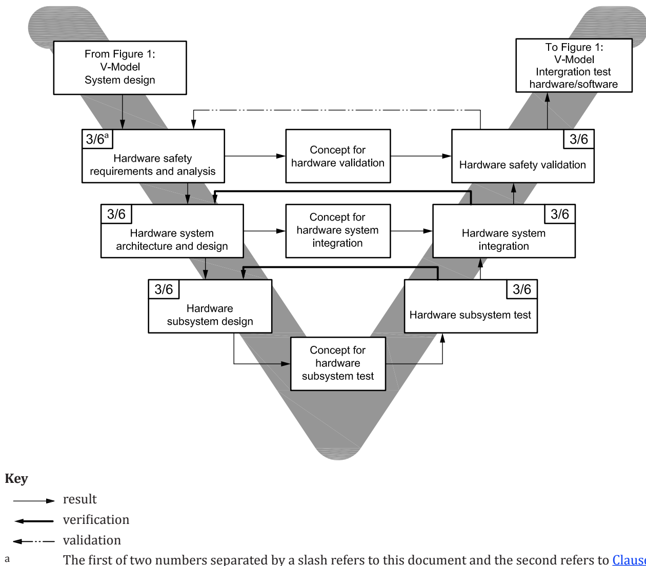
Figure 2 — Hardware development V-model
