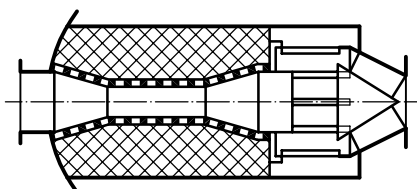
e) Silencer with spark arrestor
