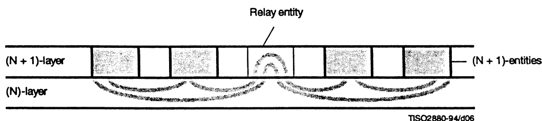
Figure 6 — Communication through a relay
