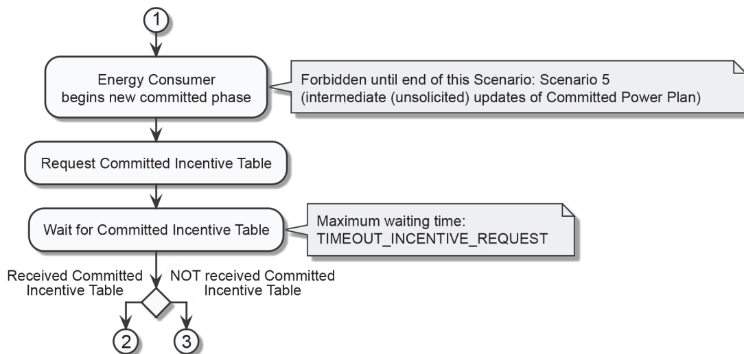
Figure 17 – Activity begin diagram of Scenario 2
