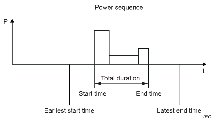
Figure 11 – Further possible properties of a scheduled power sequence
