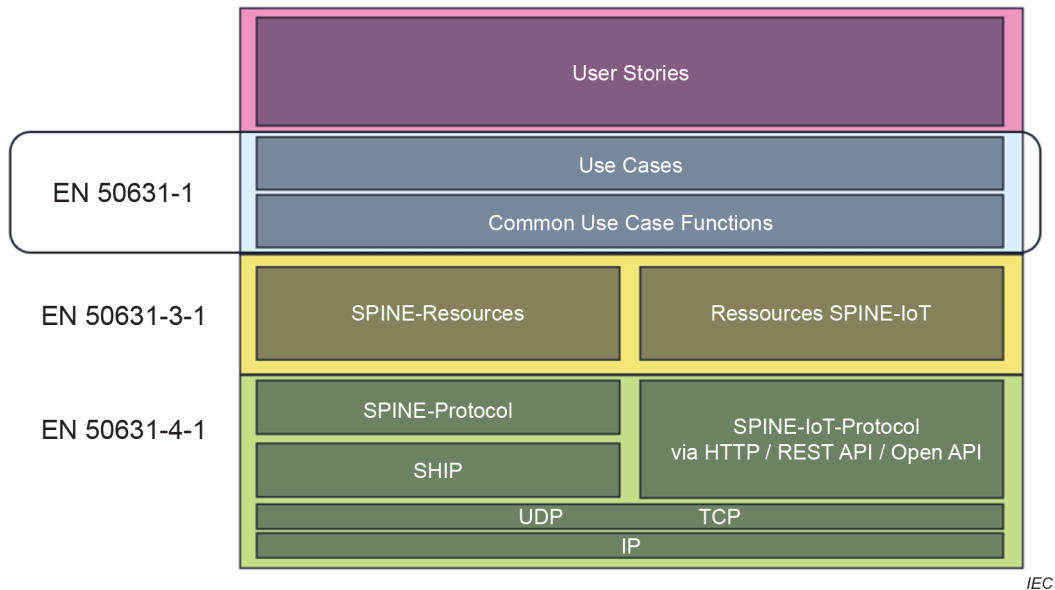
Figure 6 – Planned application of IEC 63510 series using SPINE and SHIP
