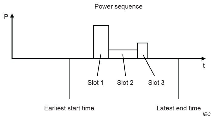
Figure 10 – Power sequence: P(t) (power-over-time) modelling with slots and time constraints
