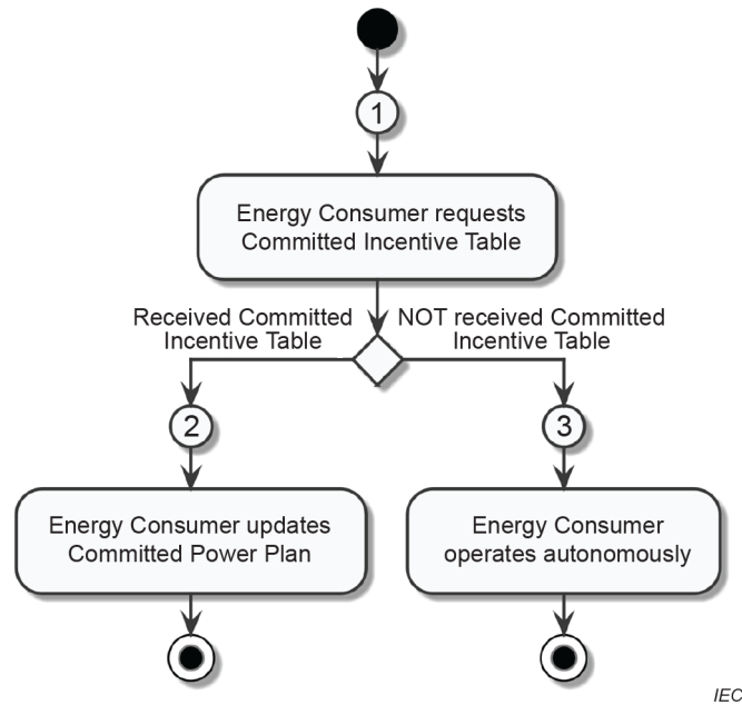
Figure 16 – Overview of Scenario 2 activity
