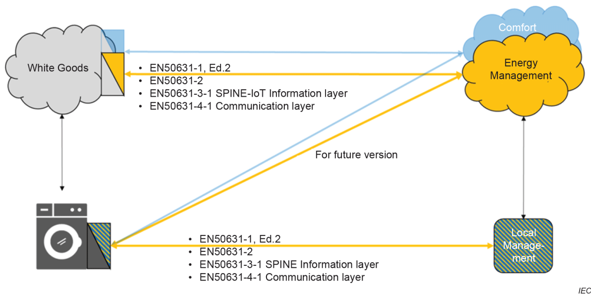
Figure 3 – Application of IEC 63510 series for the local and IoT/Cloud based operating modes
