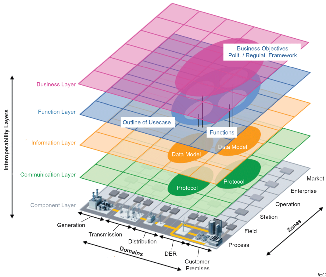
Figure 1 – SGAM Framework (from [9])
