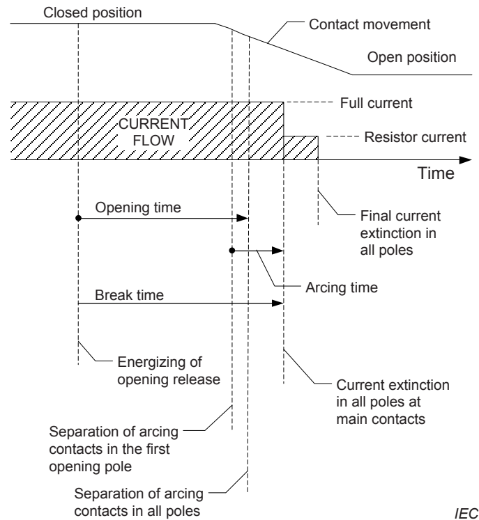
Figure 4 – Generator circuit-breaker with opening resistors – Opening operation
