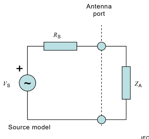
Figure 1 – Antenna feed model
