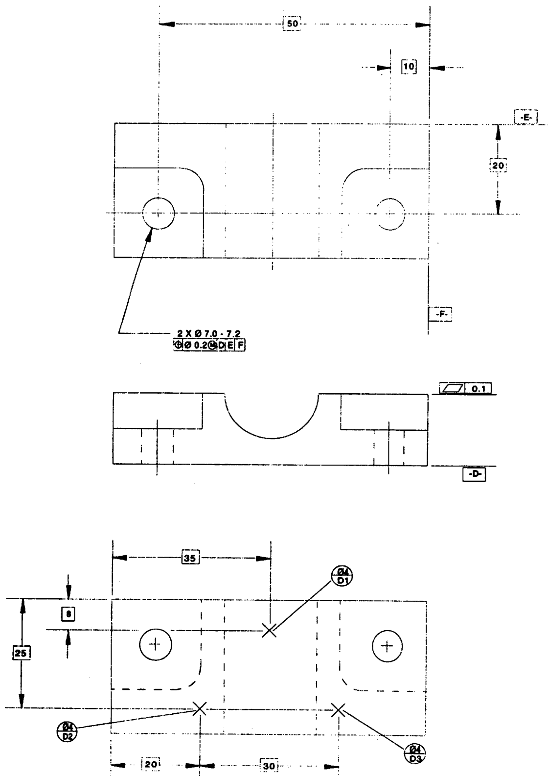
Figure 8 - Draughting callouts
