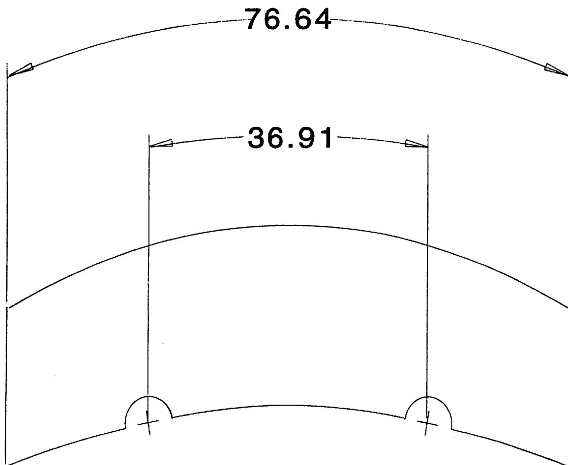
Figure 6 – Curve dimension
