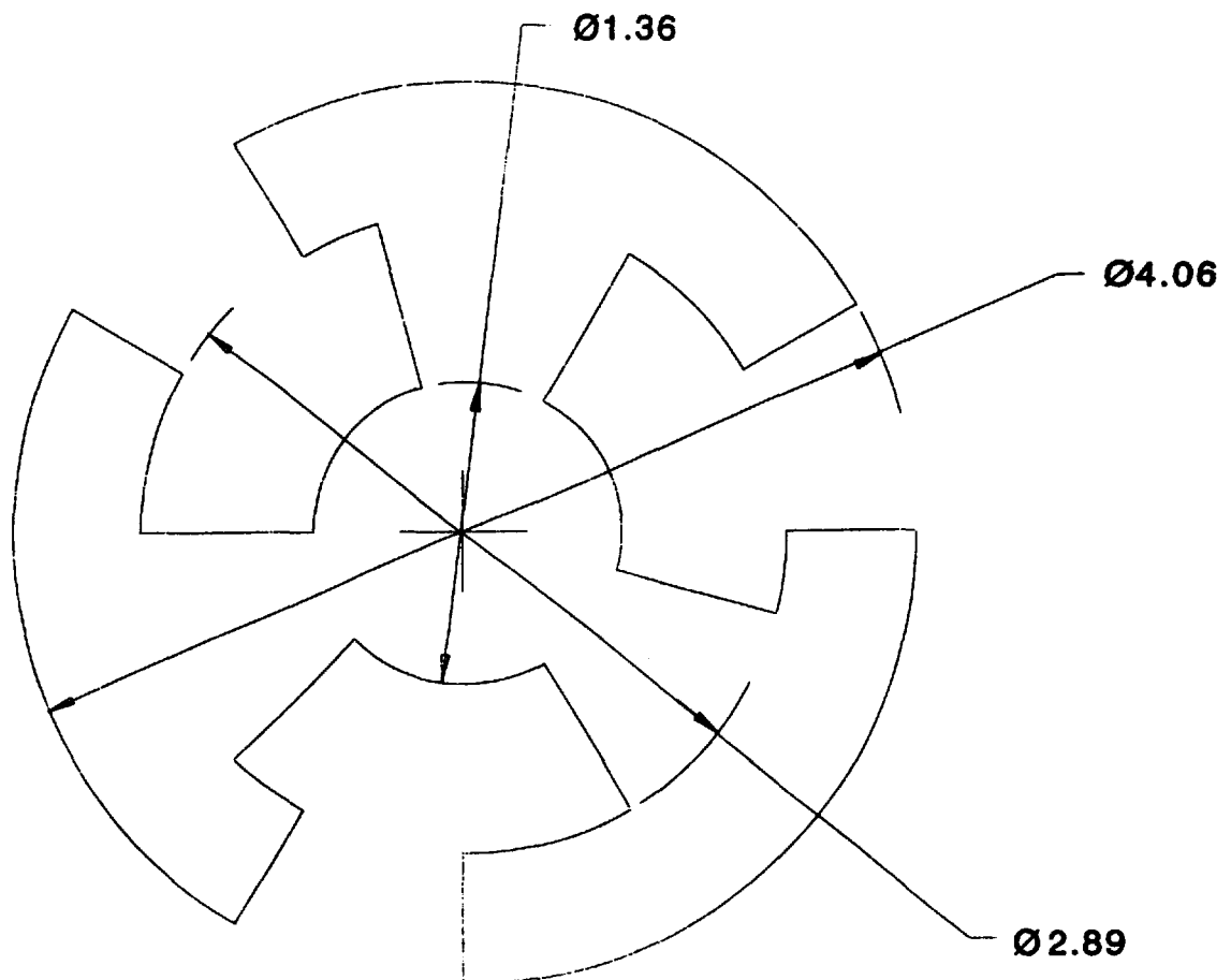
Figure 7 – Diameter dimension
