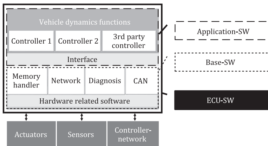
Figure 1 — Subsets of a controller
