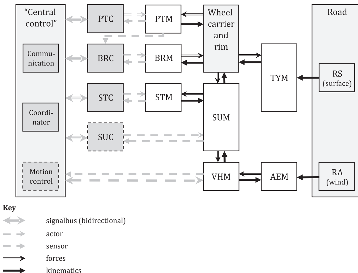
Figure 2 — Top-level model architecture
