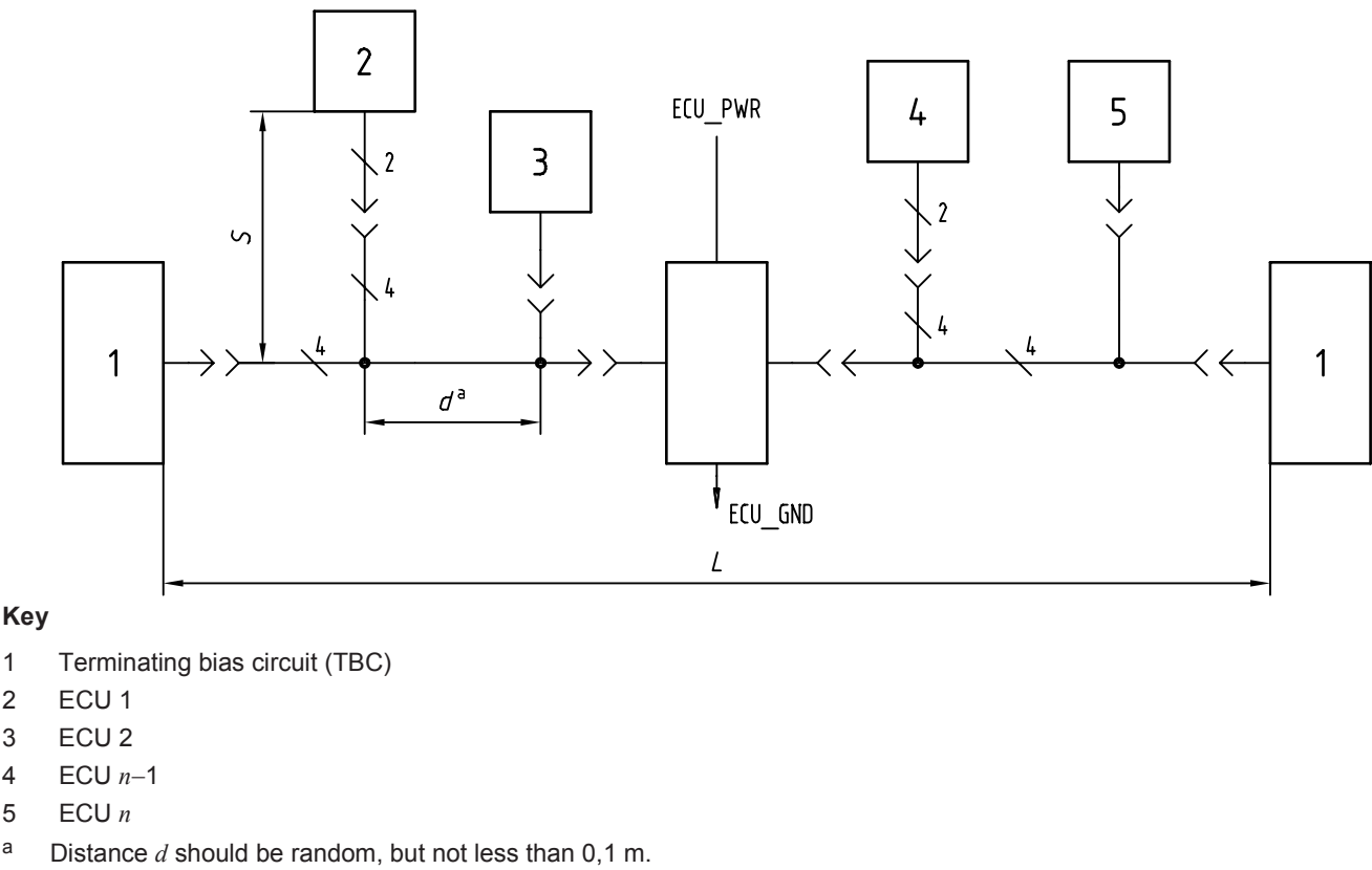
Figure 5 — Topology of bus-segment wiring
