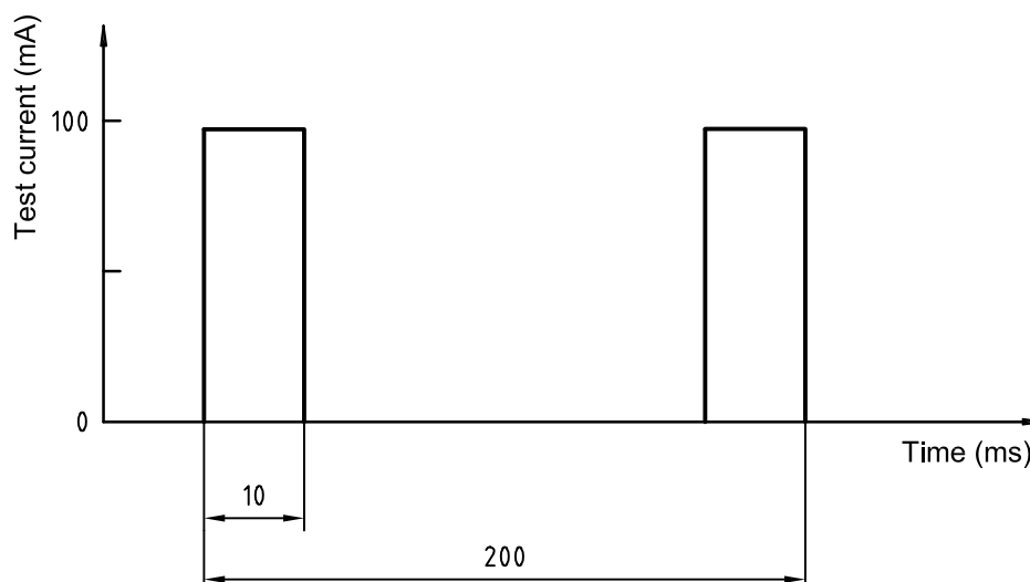
Figure 2 — Example of a test current for environmental simulation
