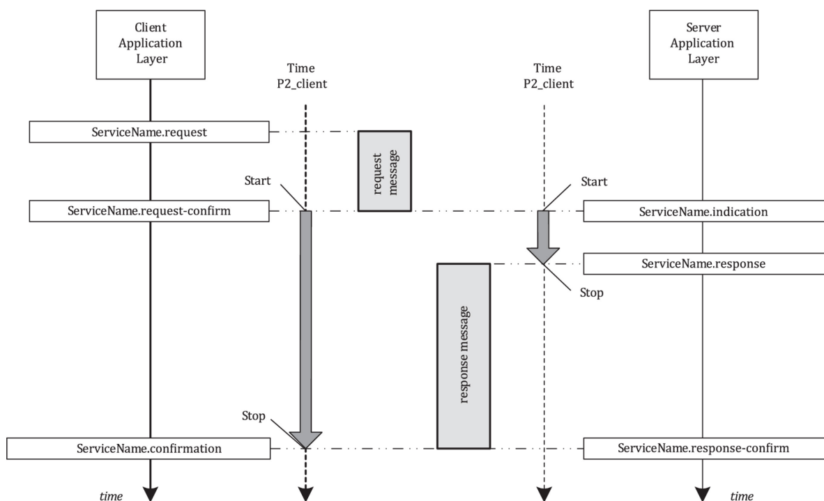
Figure 3 — Application layer service primitives – Confirmed service
