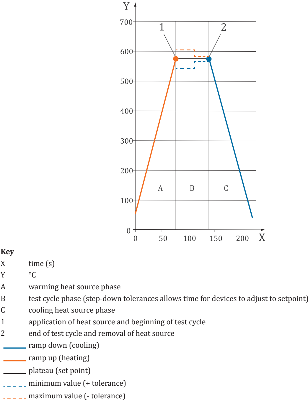
Figure 1 — Temperature-time-diagram of the test cycle with set point curve and allowed tolerances
