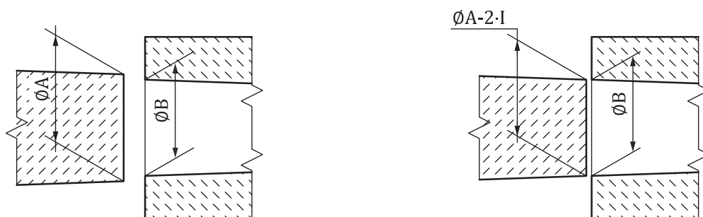
a) MISCONNECTION prevented by interference b) If \varnothing A is reduced by 2 \cdot I , it equals \varnothing B and the MISCONNECTION is possible
