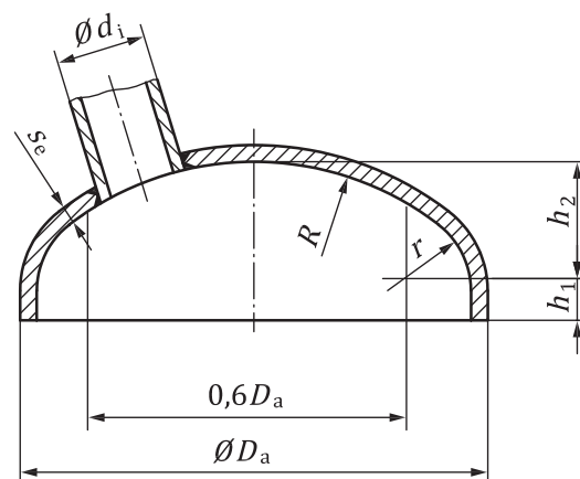
b) Dished end with nozzle
