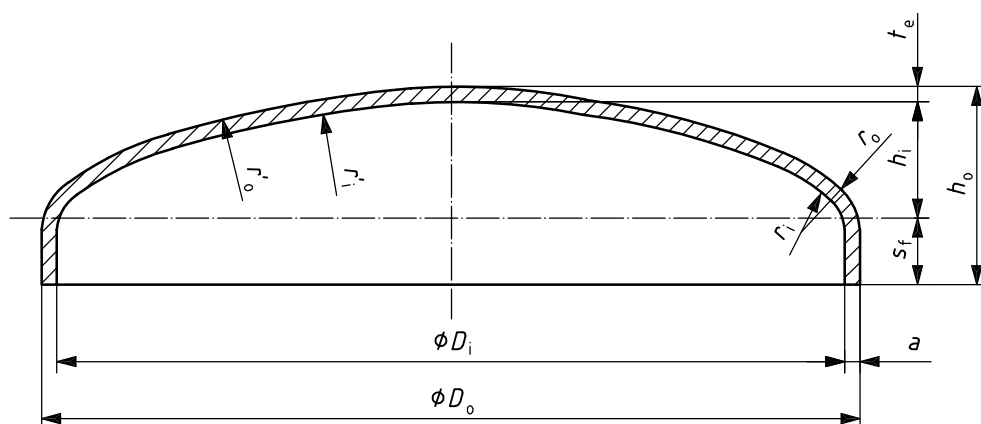
c) Torispherical
