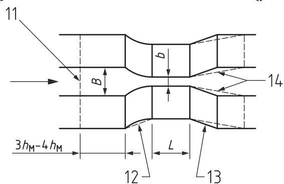
b) Plan view (example shown, no hump m_a = m , skew cylinder entrance transition)
