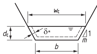
c) Section at downstream end of throat
