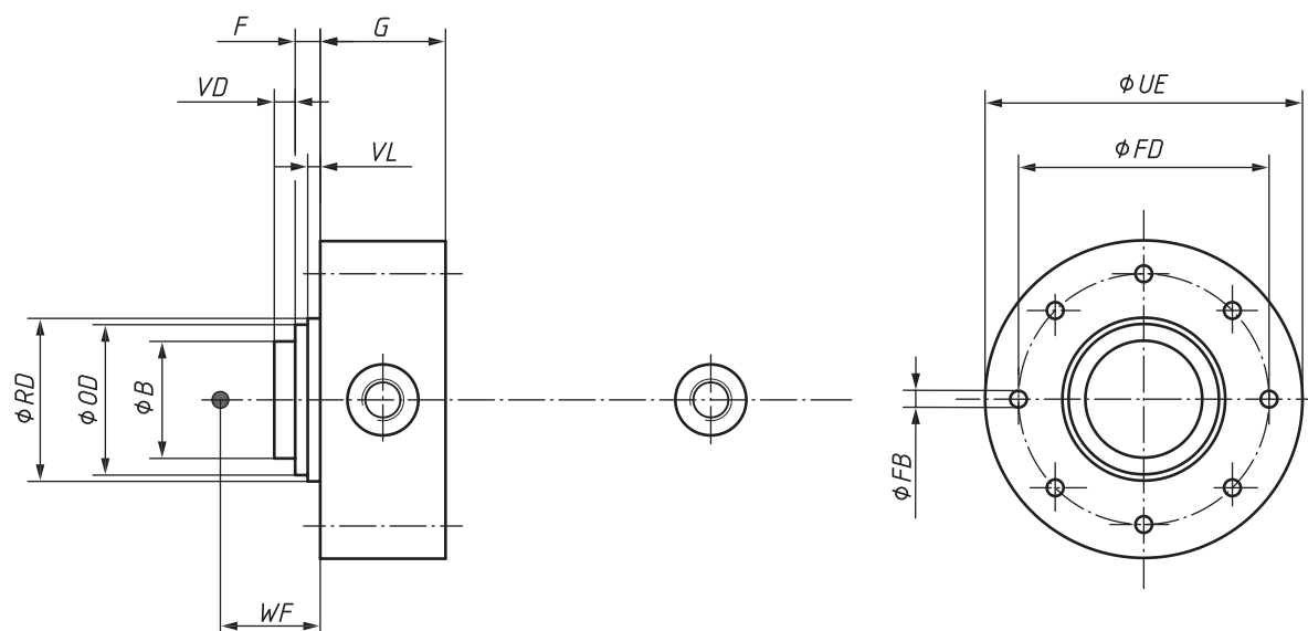
Figure 16 — ME7 — Head, round
