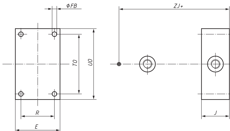
Figure 15 — ME6 — Cap, rectangular
