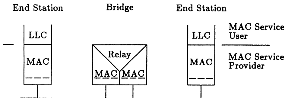
Fig 2-1 Internal Organization of the MAC Sublayer
