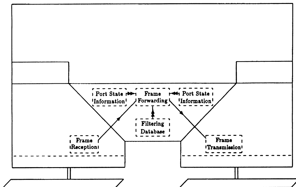
Fig 3-4 Relaying MAC Frames
