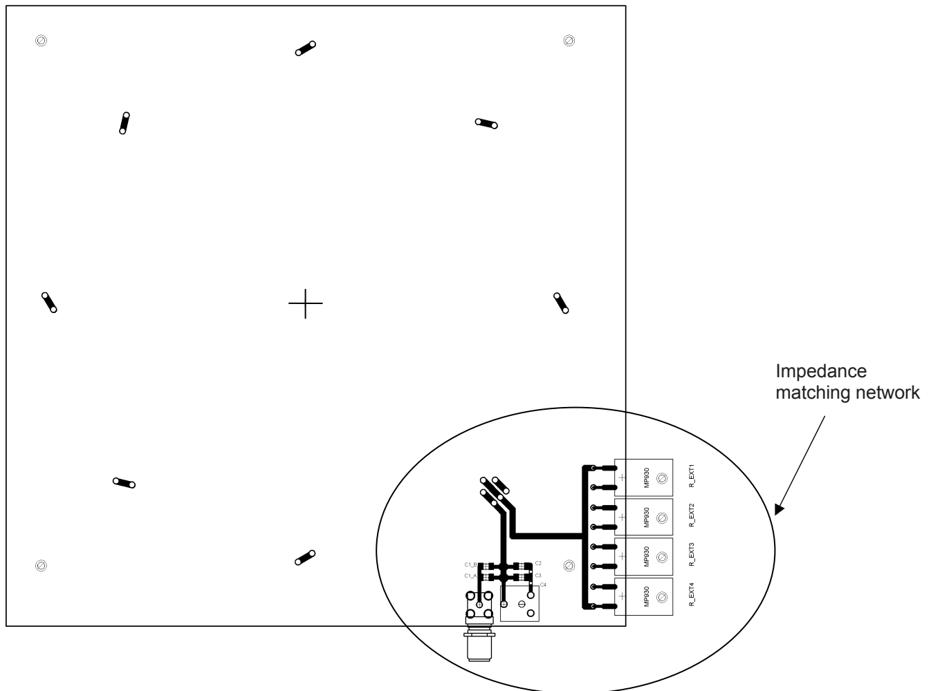
Figure A.3 — A_1 Test PCD antenna 1 A_1 layout including impedance matching network A_4 for bit rates higher than fc/128 A_4 (View from front)
