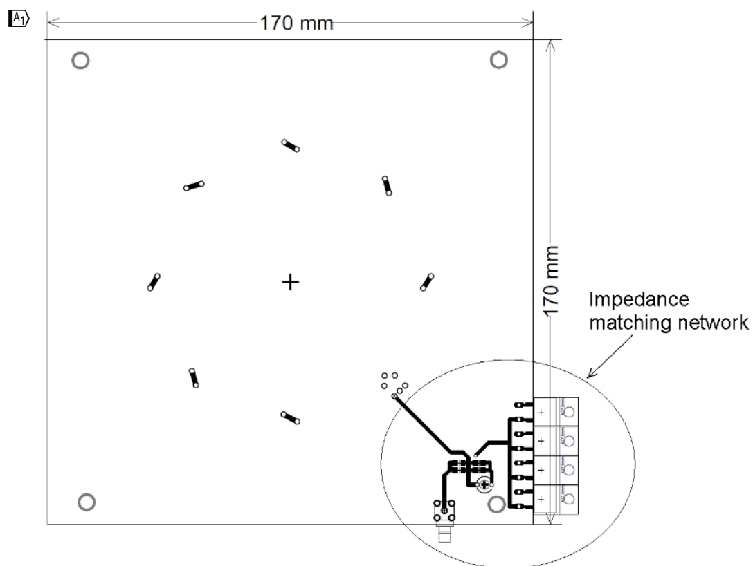
Figure A.7 — Test PCD antenna 2 layout including impedance matching network (view from front)
