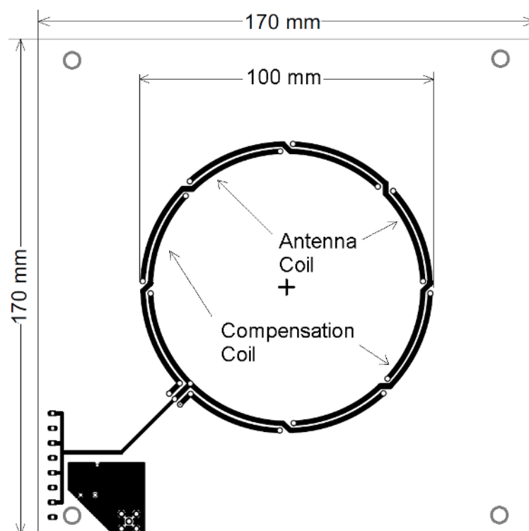
Figure A.8 — Test PCD antenna 2 layout including impedance matching network (view from back) (A1)
