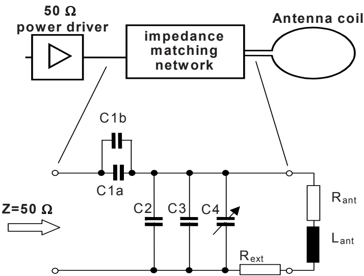
Figure A.9 — Impedance matching network 2
