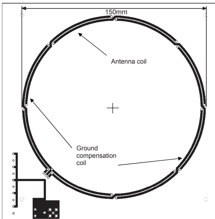
Figure A.2 — A1 Test PCD antenna1 A1 layout including impedance matching network for a bit rate of f_c/128 (View from back)
