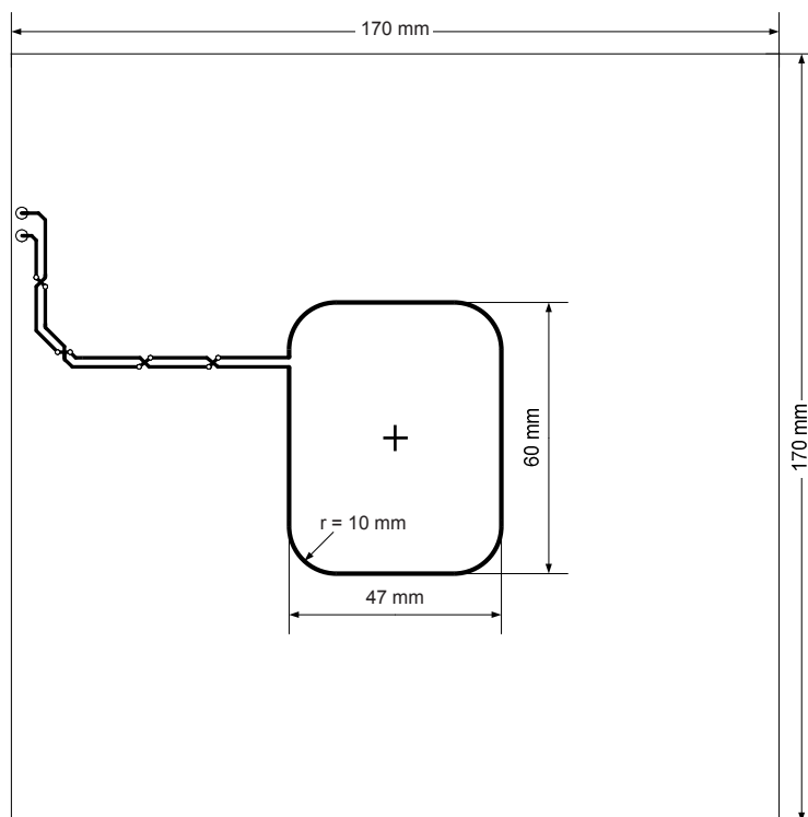
Figure C.2 — Layout for sense coils 2 (a and b) A1
