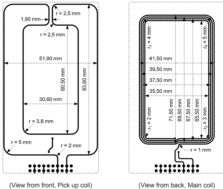
Figure D.1 — Reference PICC 1 Pick up coil and Main coil layouts
