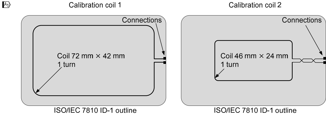
Figure 1 — Calibration coils 1 and 2
