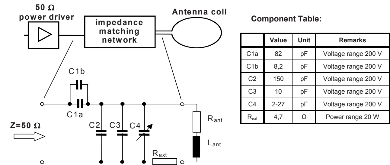
Figure A.6 — Impedance matching network \text{A}_4 for bit rates higher than fc/128\ \text{A}_4
