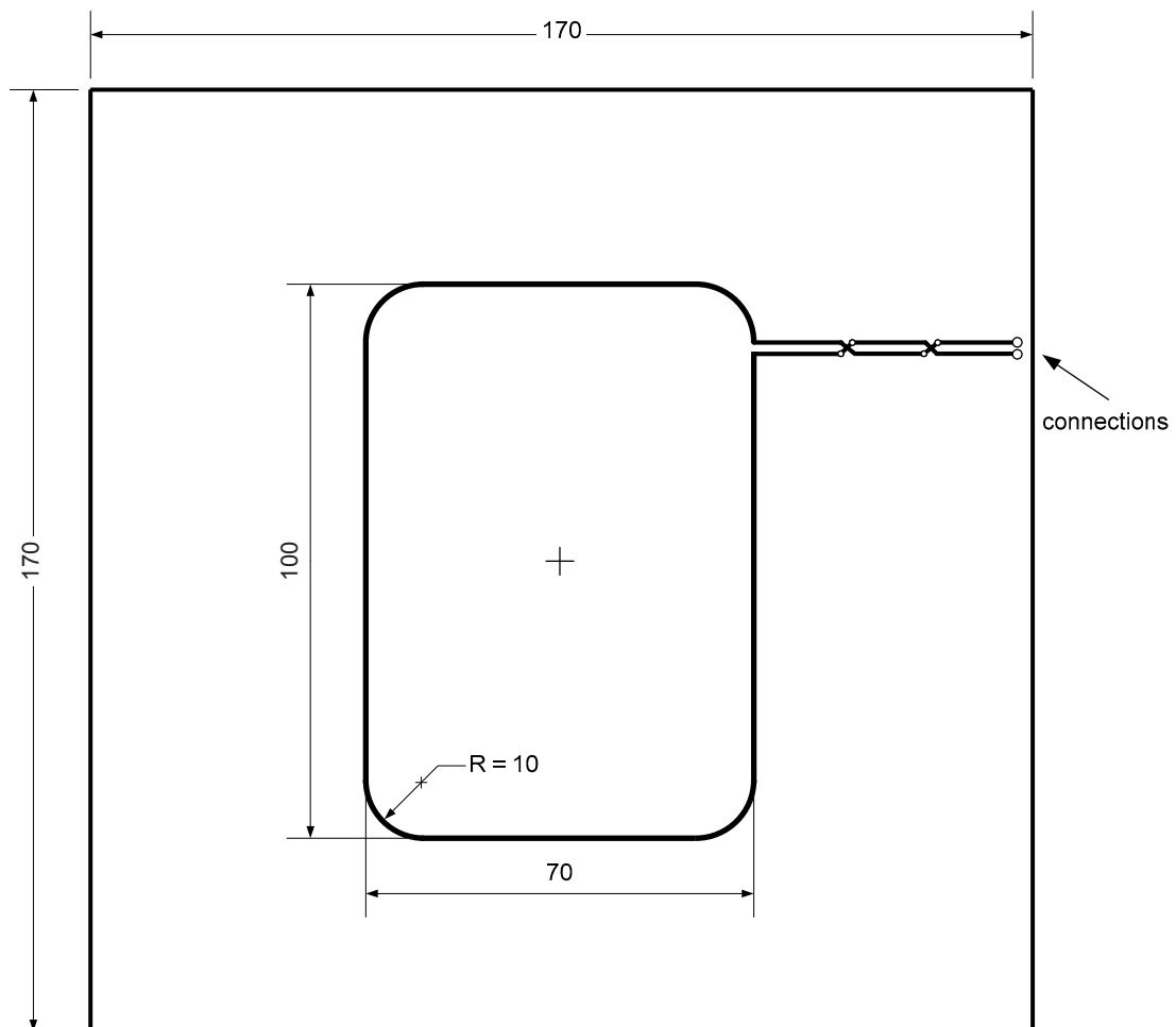
A1 Figure C.1 — Layout for sense coils 1 (a and b) A1
