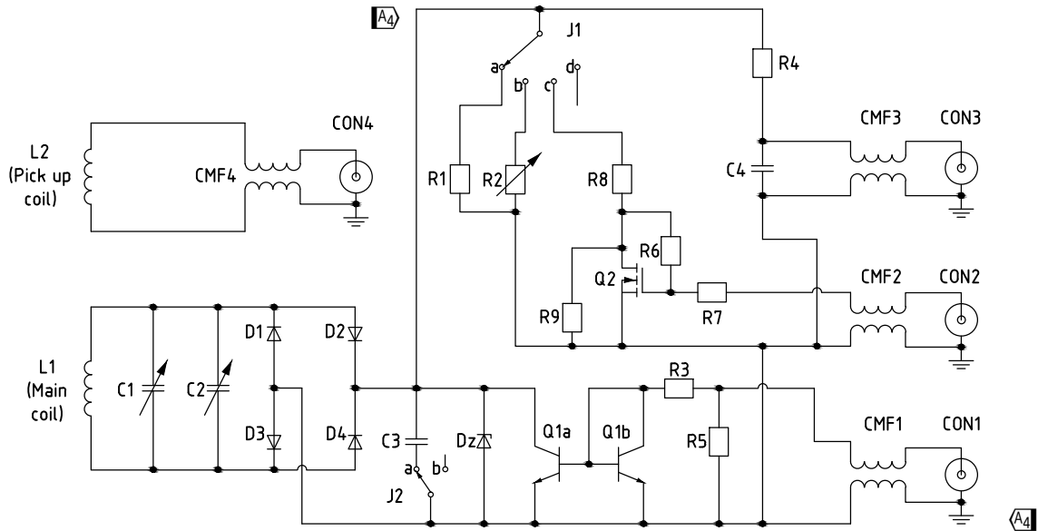
Figure 5 — Reference PICC circuit diagram
