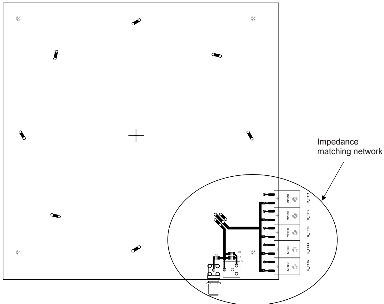
Figure A.1 — A1 Test PCD antenna 1 A1 layout including impedance matching network for a bit rate of fc/128 (View from front)
