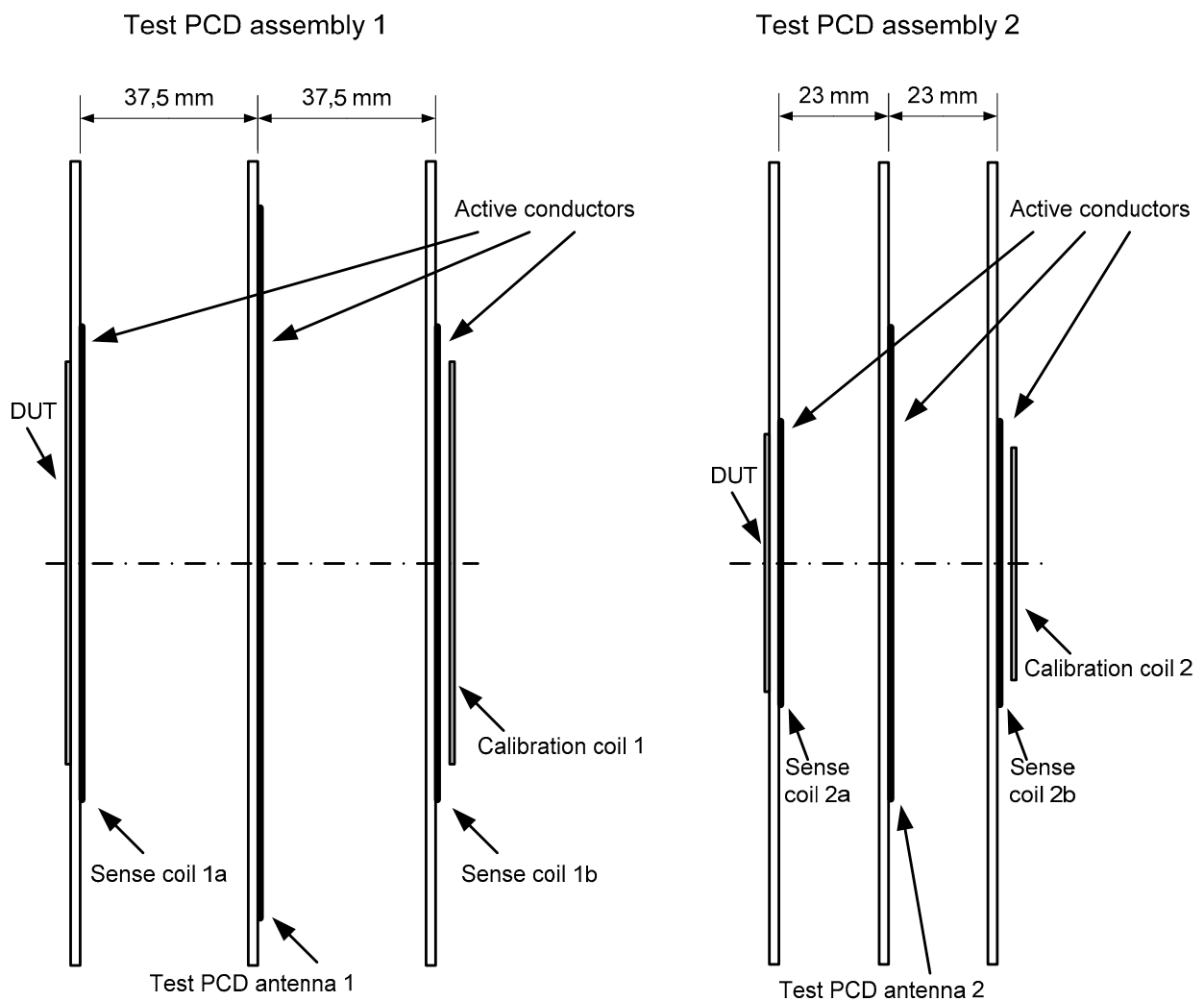
Figure 3 — Test PCD assembly 1 and test PCD assembly 2 A1
