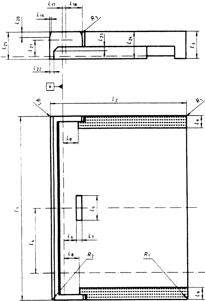
Figure 6 — Top side, lid closed
