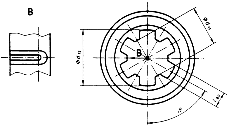
Figure 15 — Top view of a hub
