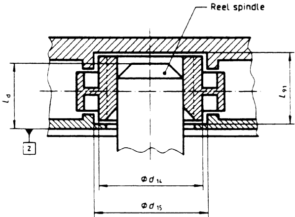
Figure 17 — Interface with the drive spindle
