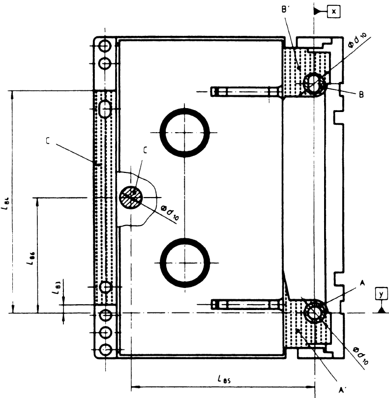
Figure 13 — Bottom side, lid and slider in open position
