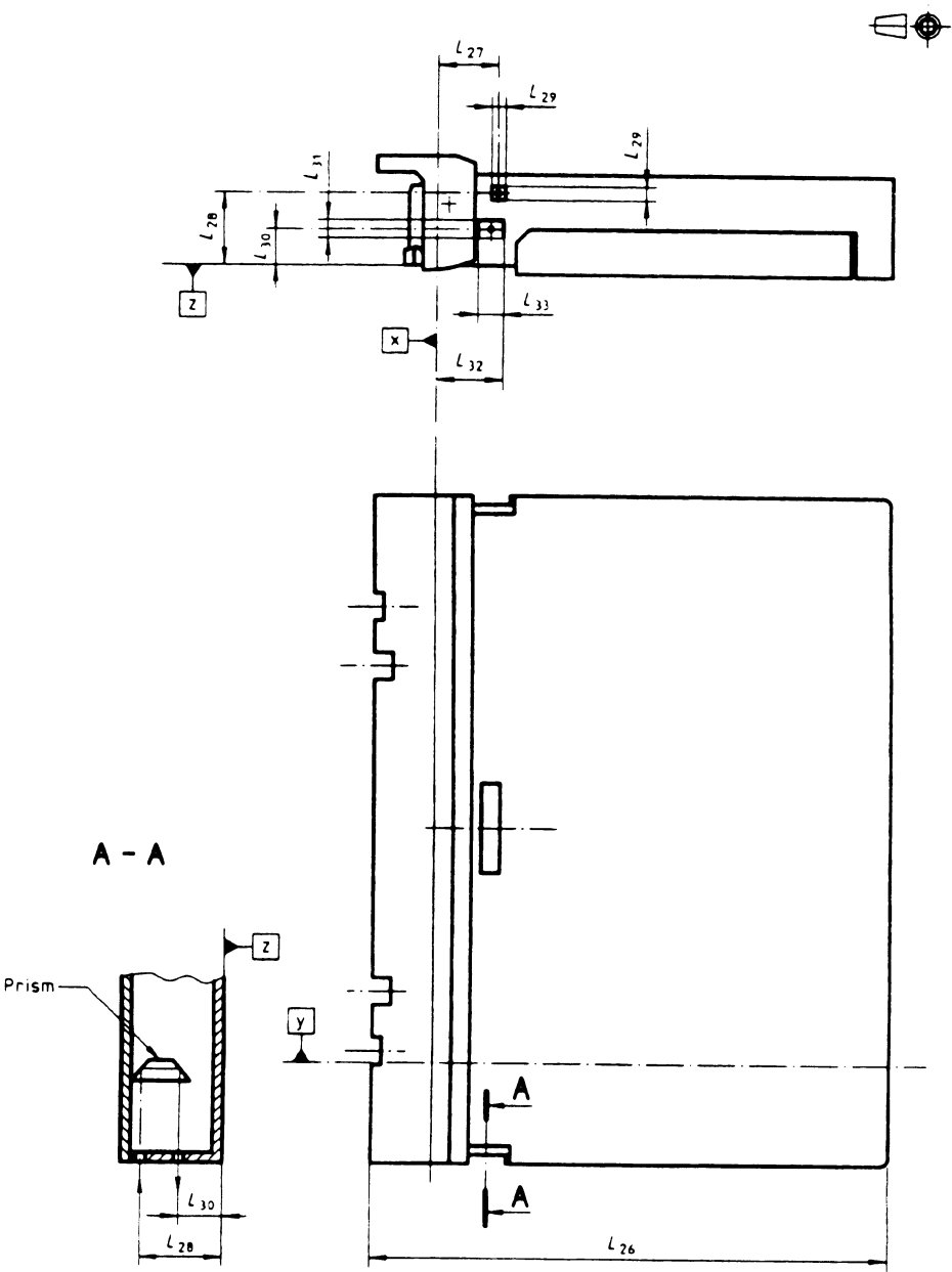
Figure 8 — Top side, lid open
