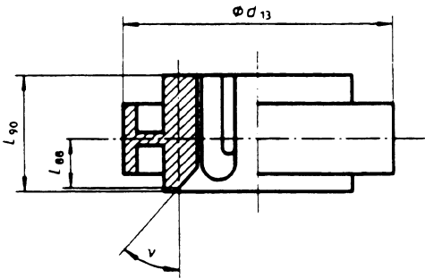
Figure 16 — Side view of a hub
