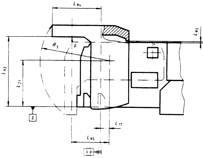
Figure 18 — Lid in completely open position
