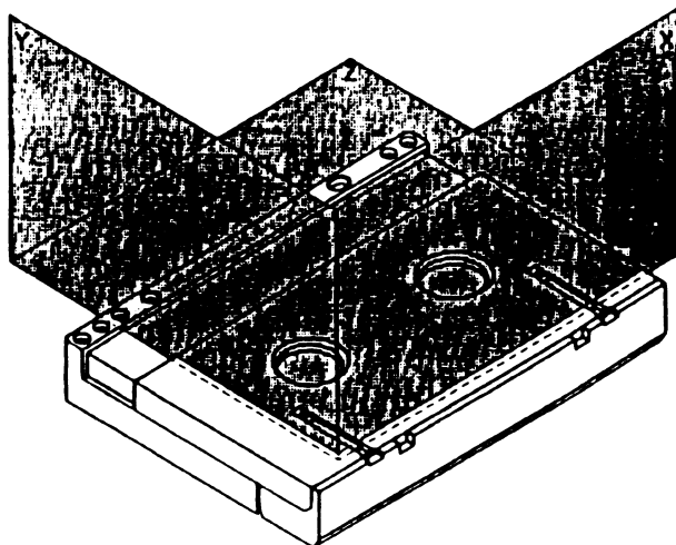
Figure 4 — Reference Planes X, Y, Z
