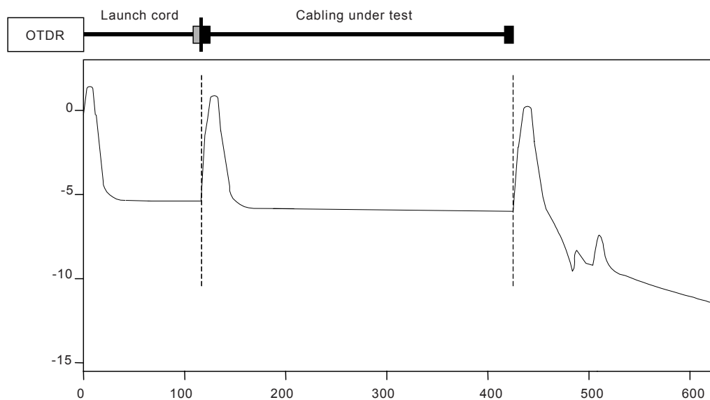
Figure 3 – OTDR characterization using a launch cord only
