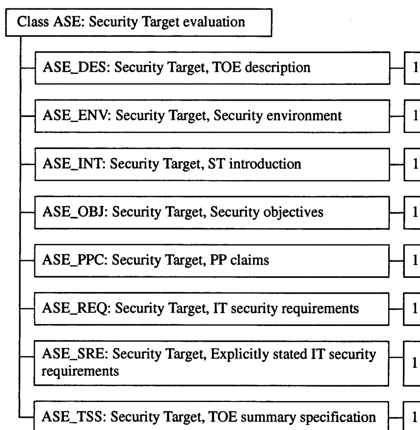
Figure 5.1 - Security Target evaluation class decomposition
