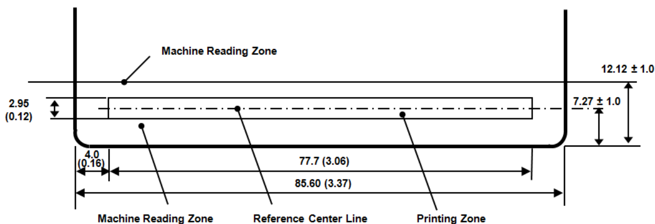
Figure Amd.1-1 — Location of 1 line MRZ at the bottom of the IDL (not to scale)
