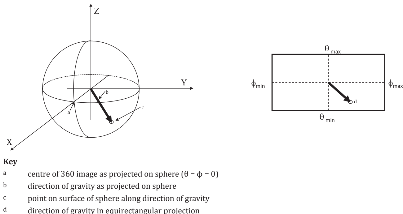
Figure 6 — Representation for direction of gravity for non-upright camera
