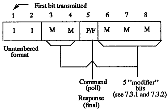
Figure 6 - Unnumbered format of control field bits
