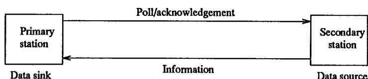
Figure 2 — Unbalanced data link configuration (case 2)
