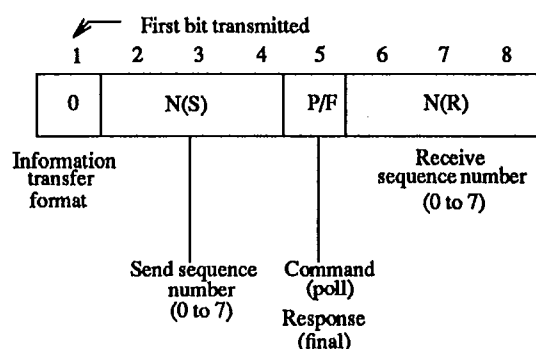
Figure 4 - Information transfer format of control field bits
