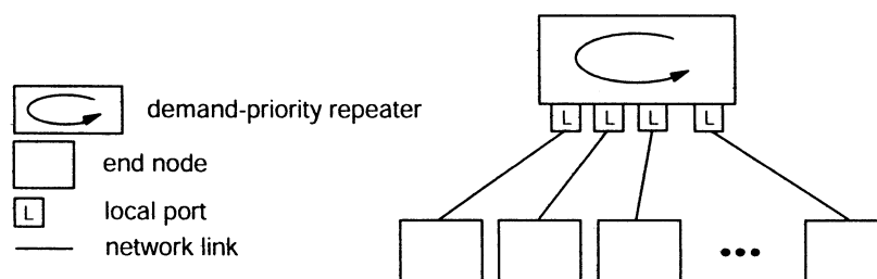
Figure 6-1—A single-repeater network topology
