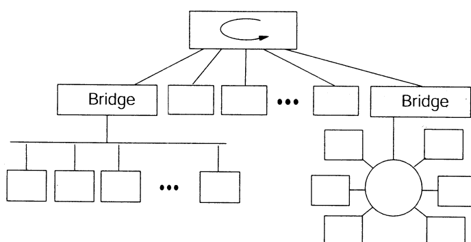
Figure 6-3—A demand-priority network interconnected with other LANs
