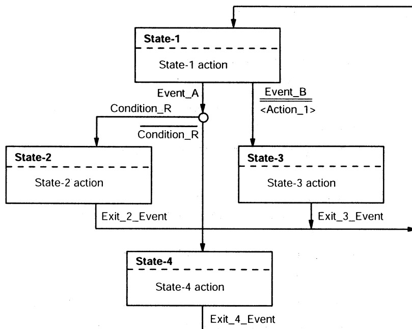
Figure 5-3—Example state machine diagram
