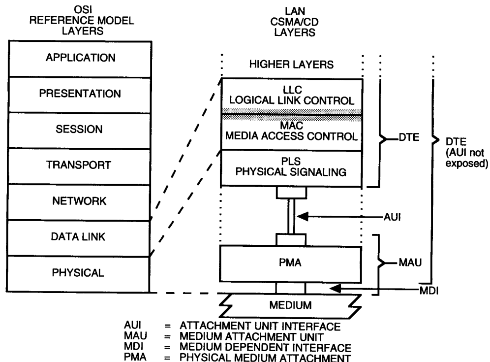
Fig 2-1 Service Specification Relation to the LAN Model
