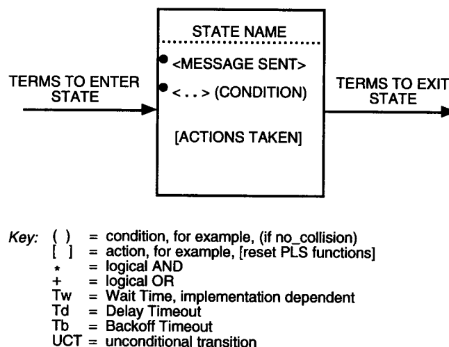
Fig 1-2 State Diagram Notation Example
