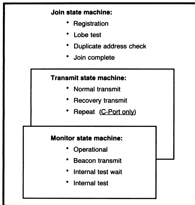
Figure 9-3—Join, Transmit, and Monitor FSM interaction
