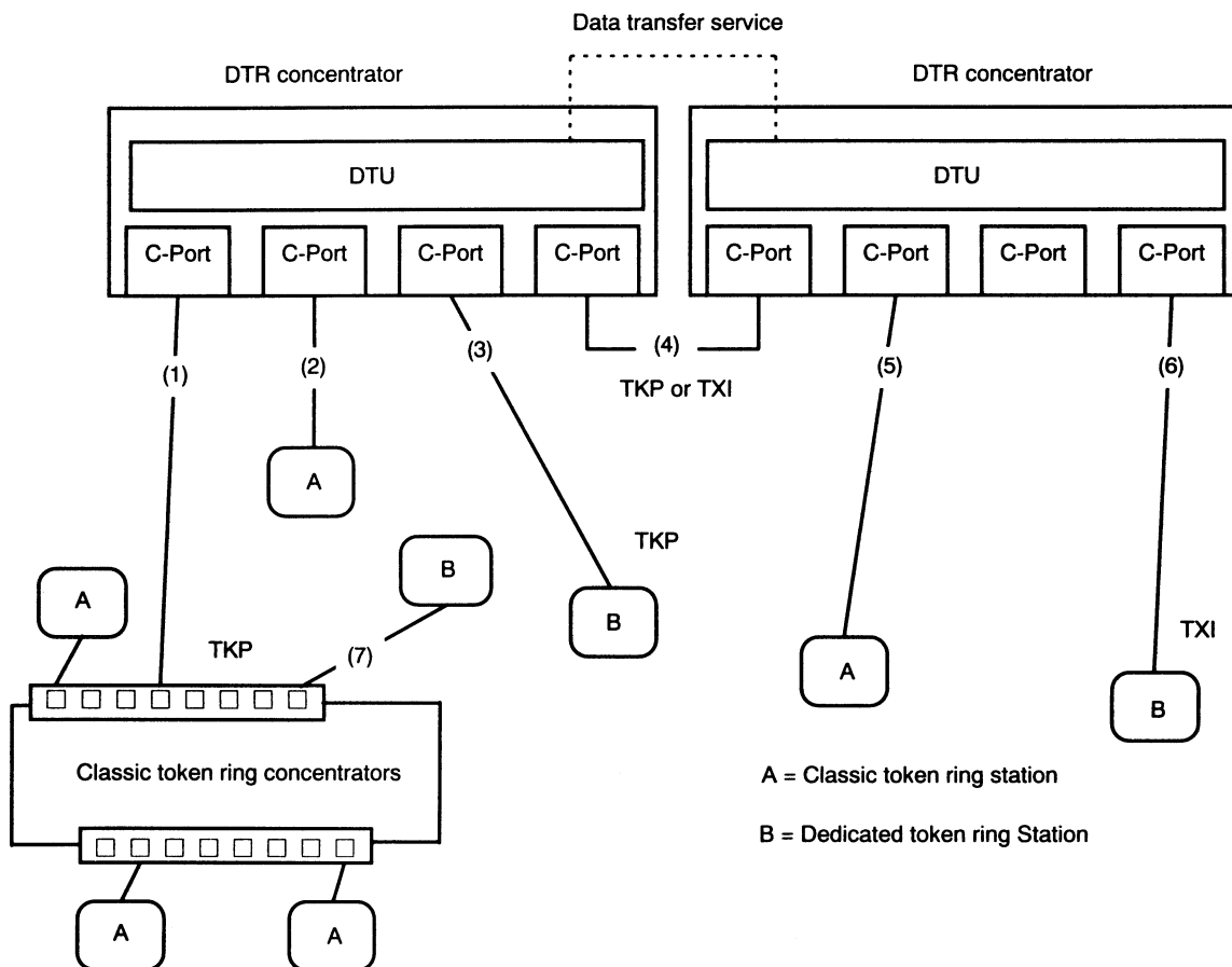
Figure 2.5-1—DTR network
