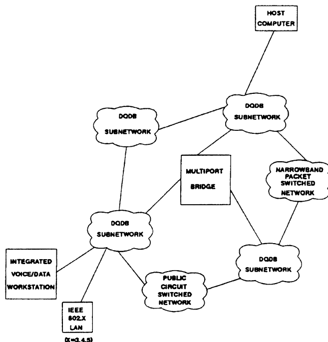
Figure A — DQDB metropolitan area network
