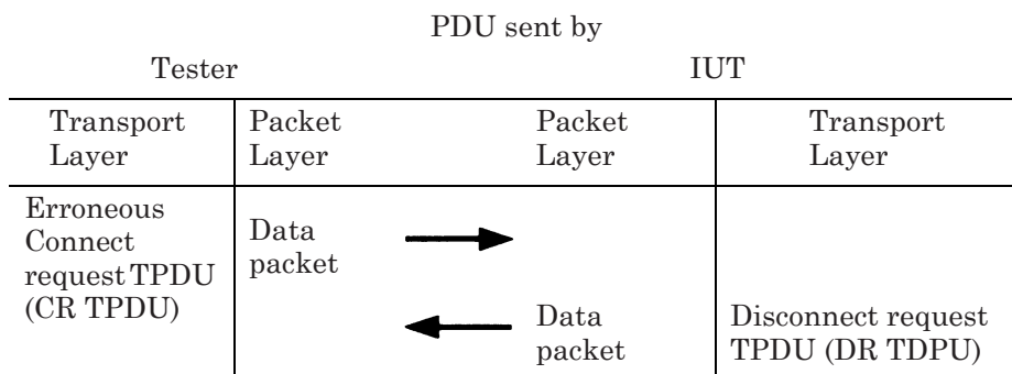
Figure 4 — Example of the use of a Transport Layer Sub-function directly over ISO/IEC 8208 (i.e. OSI Network Layer)
