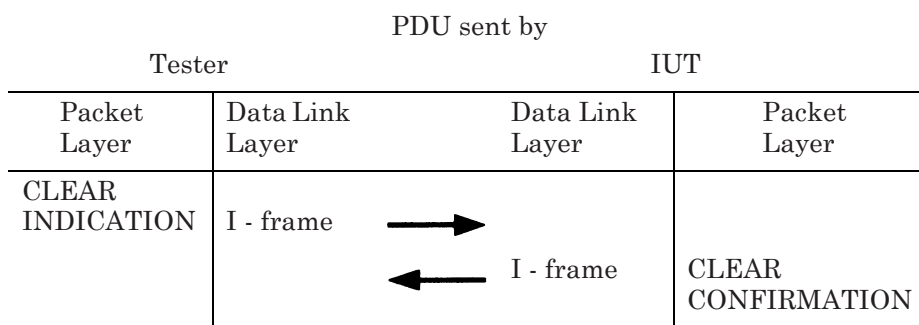
Figure 3 — Example of the use of a Packet Layer Sub-function
