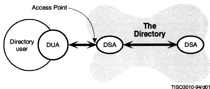
Figure 1 – Directory Interactions
