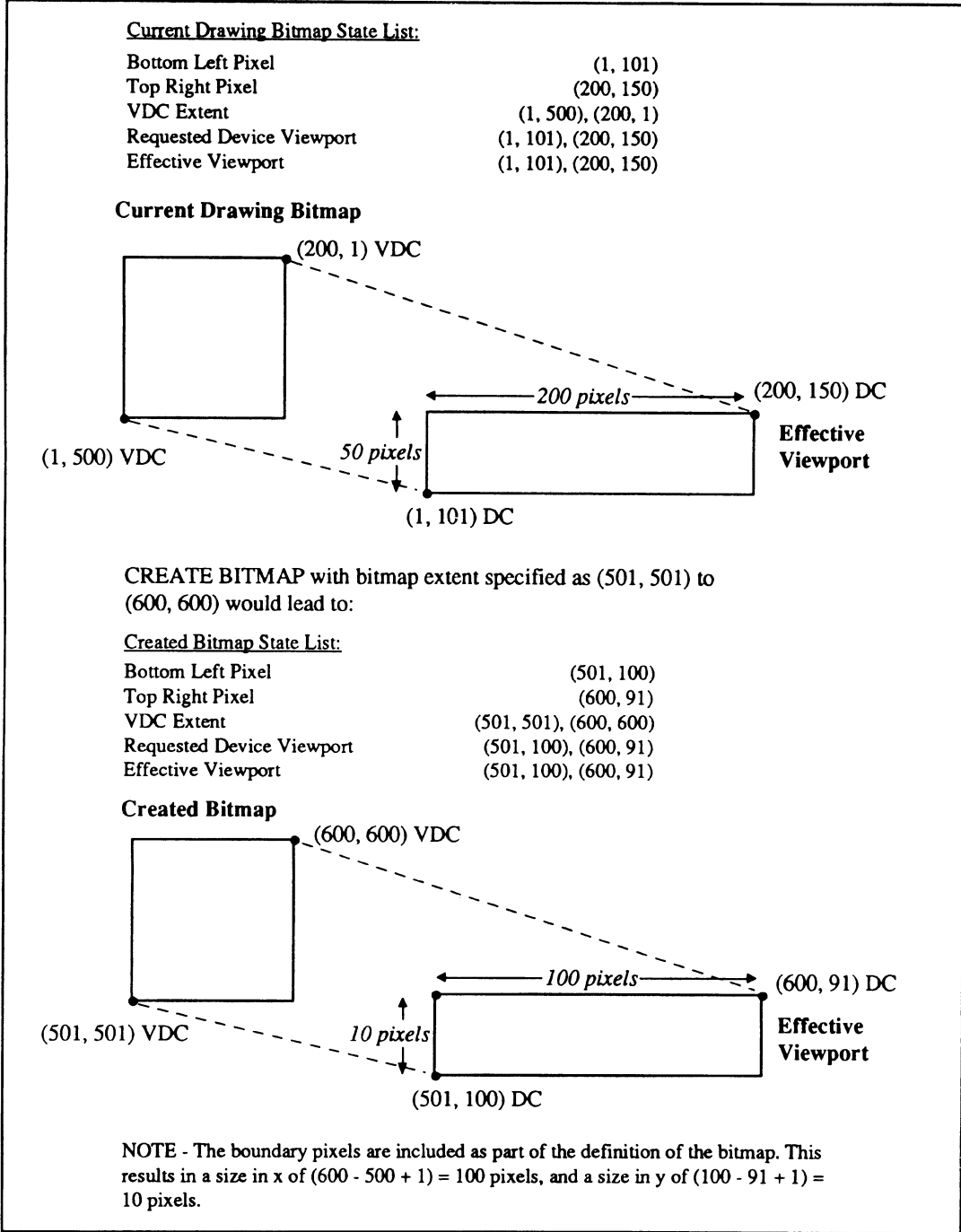
Figure 5 — Creating bitmaps
