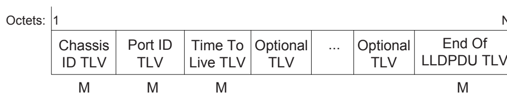
Figure 8-1—LLDPDU format
