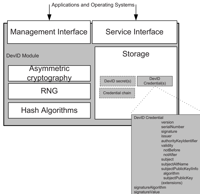
Figure 6-1— DevID components
