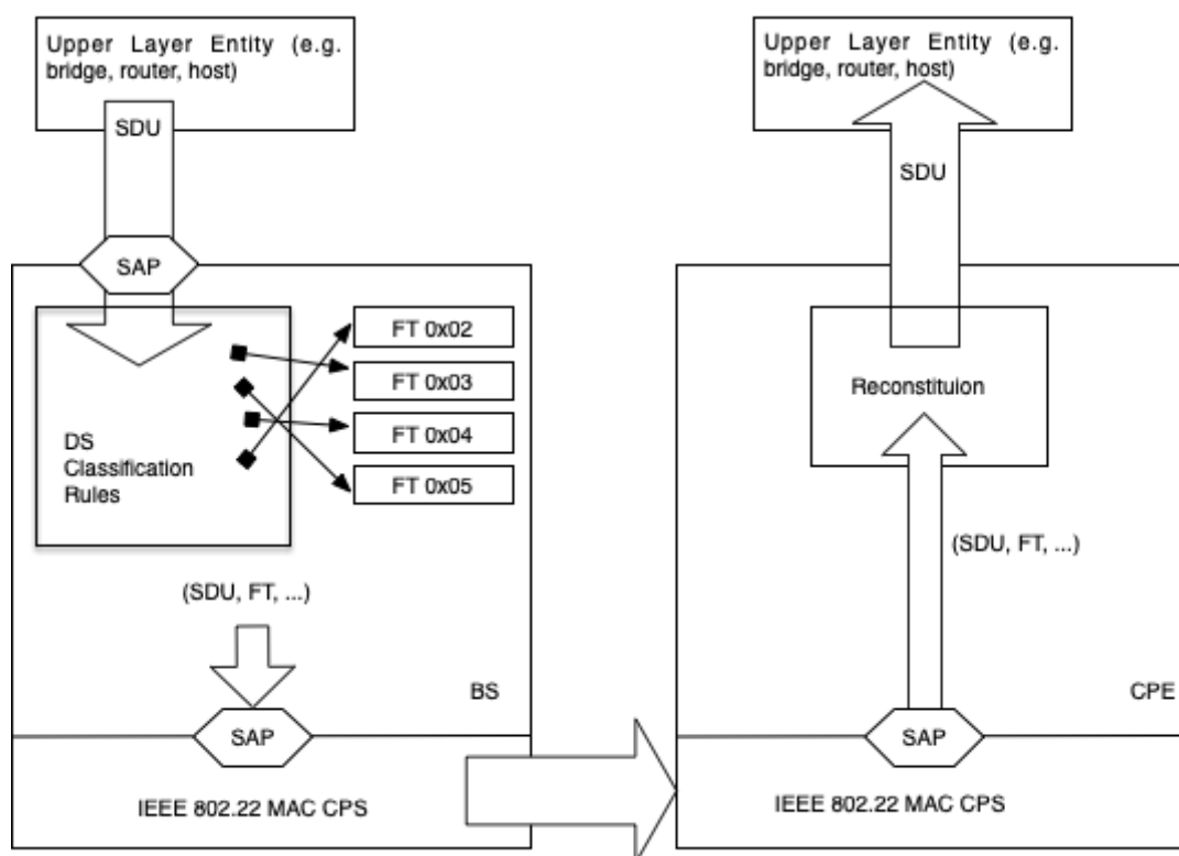
Figure 8—Classification and FT mapping (BS to CPE)
