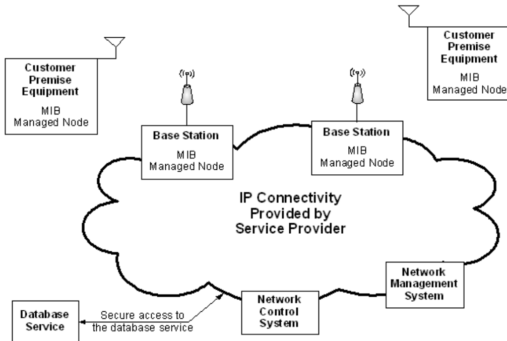
Figure 5—Management reference model
