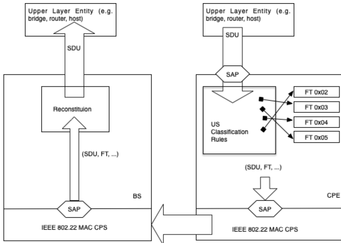
Figure 9—Classification and FT mapping (CPE to BS)
