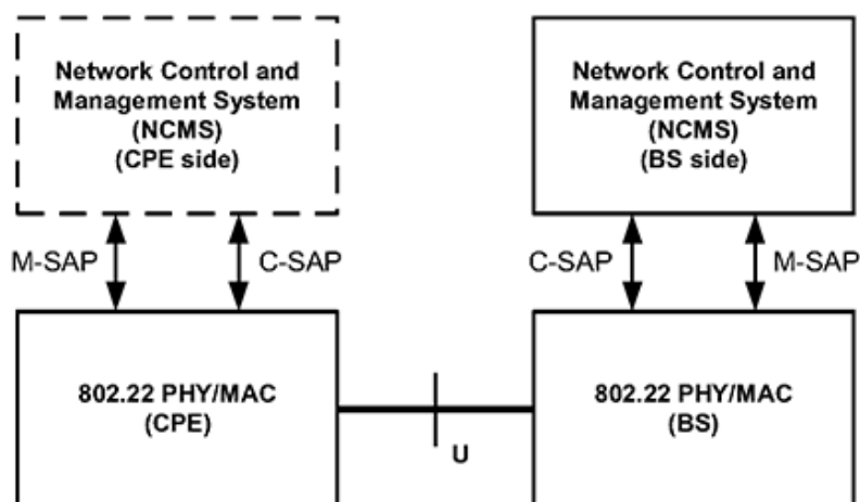
Figure 6—IEEE 802.22 Network Reference Model
