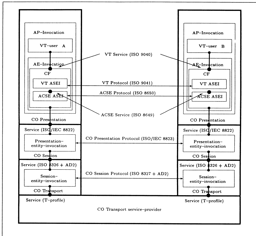
Figure 1 — Interactive VT communication between two end systems
