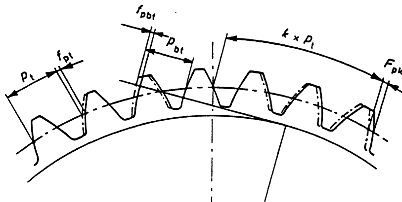
Fig. 3 Pitch ( p_t ), pitch deviation ( f_{pt} ), transverse base pitch ( p_{bt} ), transverse base pitch deviation ( f_{pbt} ), cumulative pitch ( k \times p_t , in the Fig. k=3 ), cumulative pitch deviation ( F_{pk} , in the Fig. k=3 )
