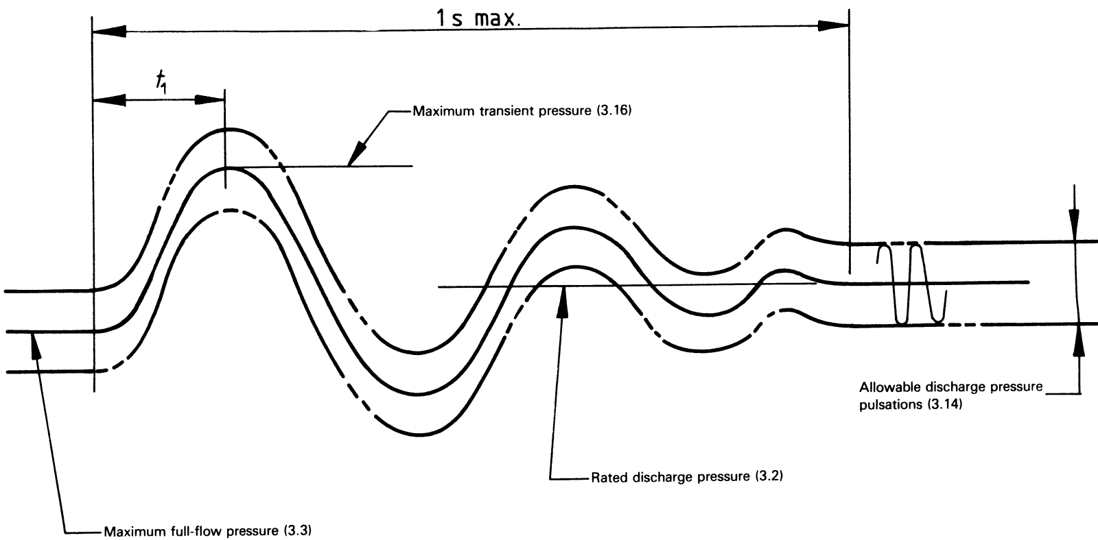
Figure 3 — Typical variation of pressure against time — Transient from maximum full-flow pressure to rated discharge pressure (zero flow)
