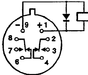
With coil transient suppression diode
