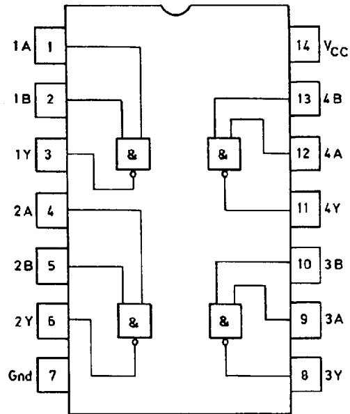
Quadrate 2-input positive Nand gates
