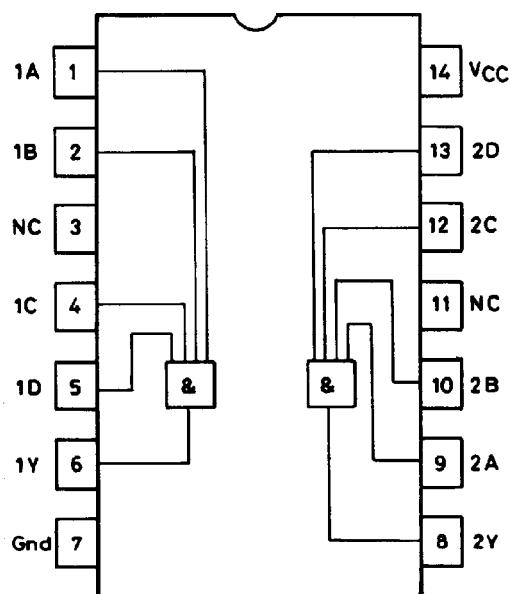
Dual 4-input positive Nand gates
