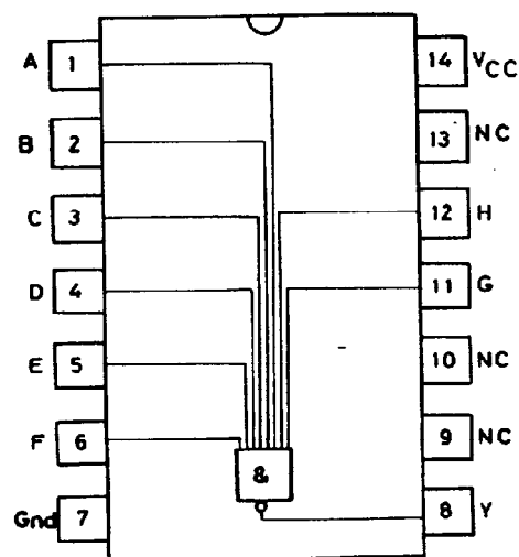
8-input positive Nand gates
