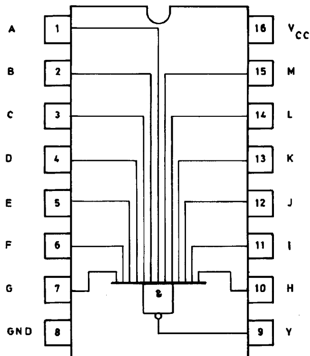
13 input positive-Nand gates
