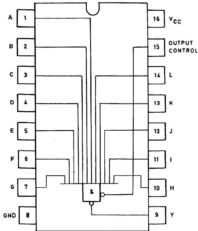
12-input positive Nand gates
