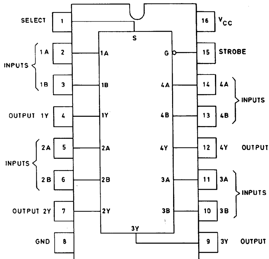
Quadruple 2 line-to-1-line data selectors/multiflexers
