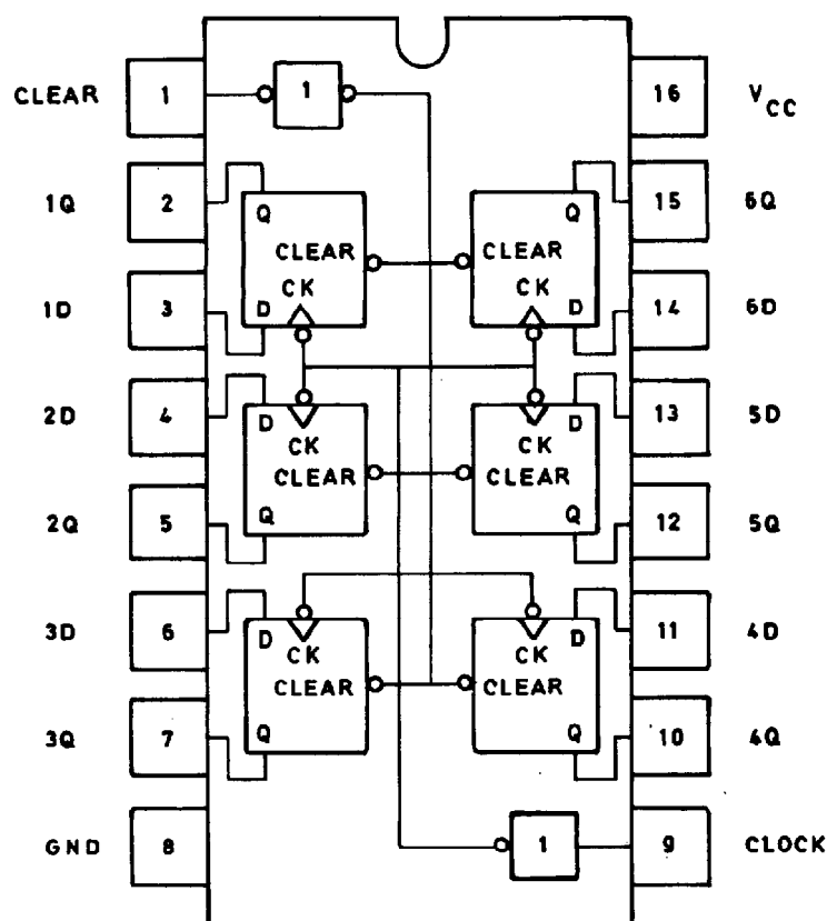
Hex D-type bistables with clear
