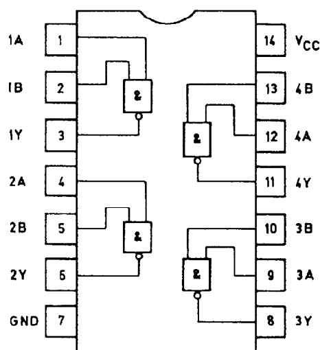
Quad 2-input Nand gates
