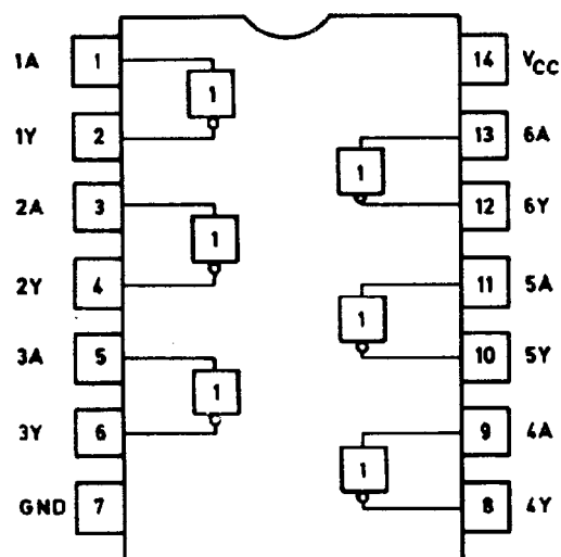
Six independent inverters each with one input
