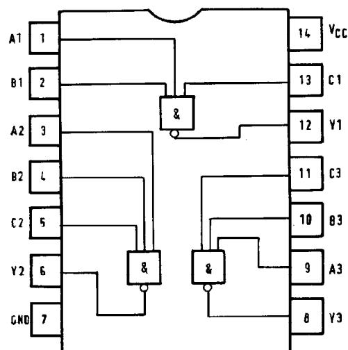
Three 3-input Nand gates with open collector outputs
