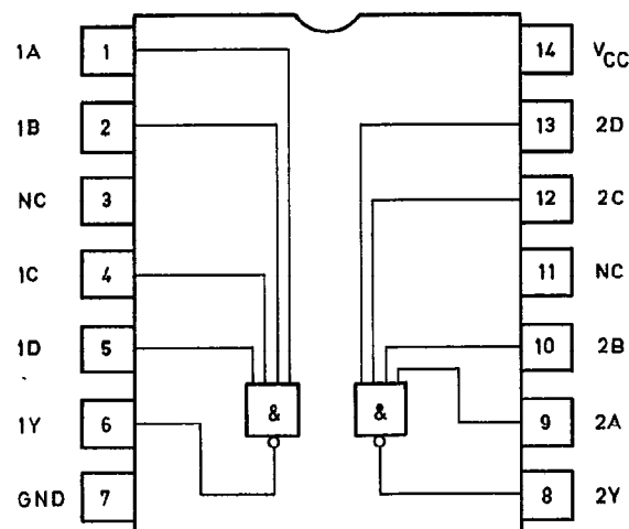
Dual 4-input Nand gates
